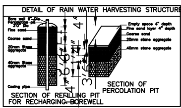
DETAIL OF RAIN WATER HARVESTING STRUCTURE
